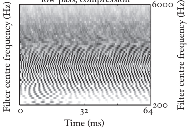
Gammatone, half-wave low-pass, compression
